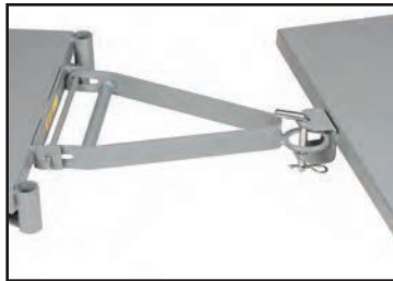
Versatile ring type wishbone coupler with 2-1/2" I.D. ring can also be used with most pintle hitches.
